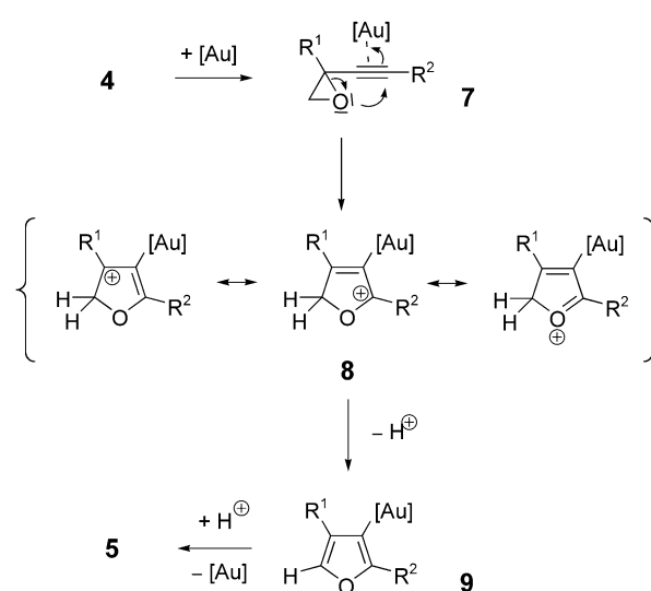
Scheme 2. Mechanistic proposal for the gold-catalyzed isomerization of 4 to 5 .
