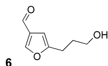
Scheme 1. Sequence to the alkynyl epoxides 4 and their gold-catalyzed isomerization to 5 .
